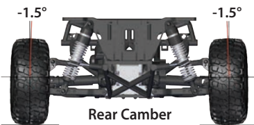
Rear Camber
